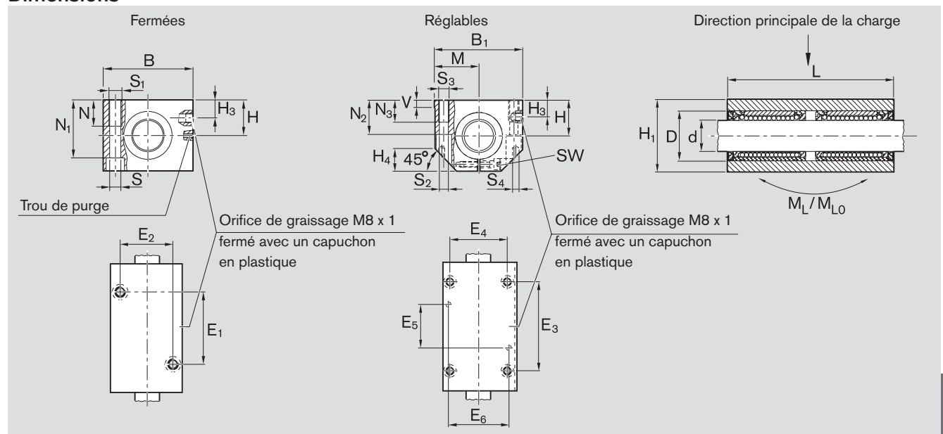
Dimensions (mm)
